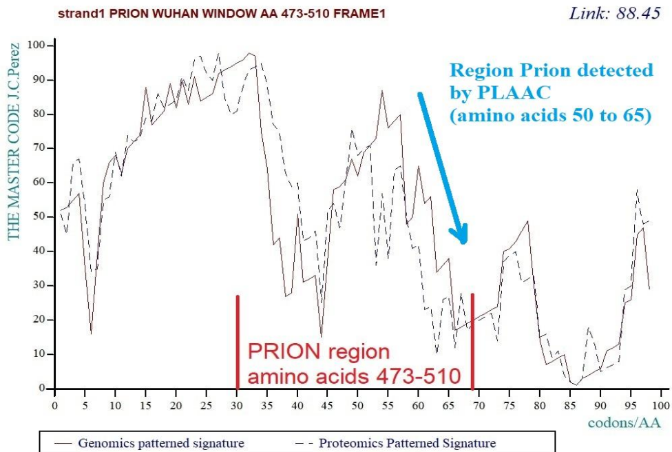
Figure 13 – PLAAC evidence of a Prion region in the 100 amino acids region overlapping Wuhan Prion region.
